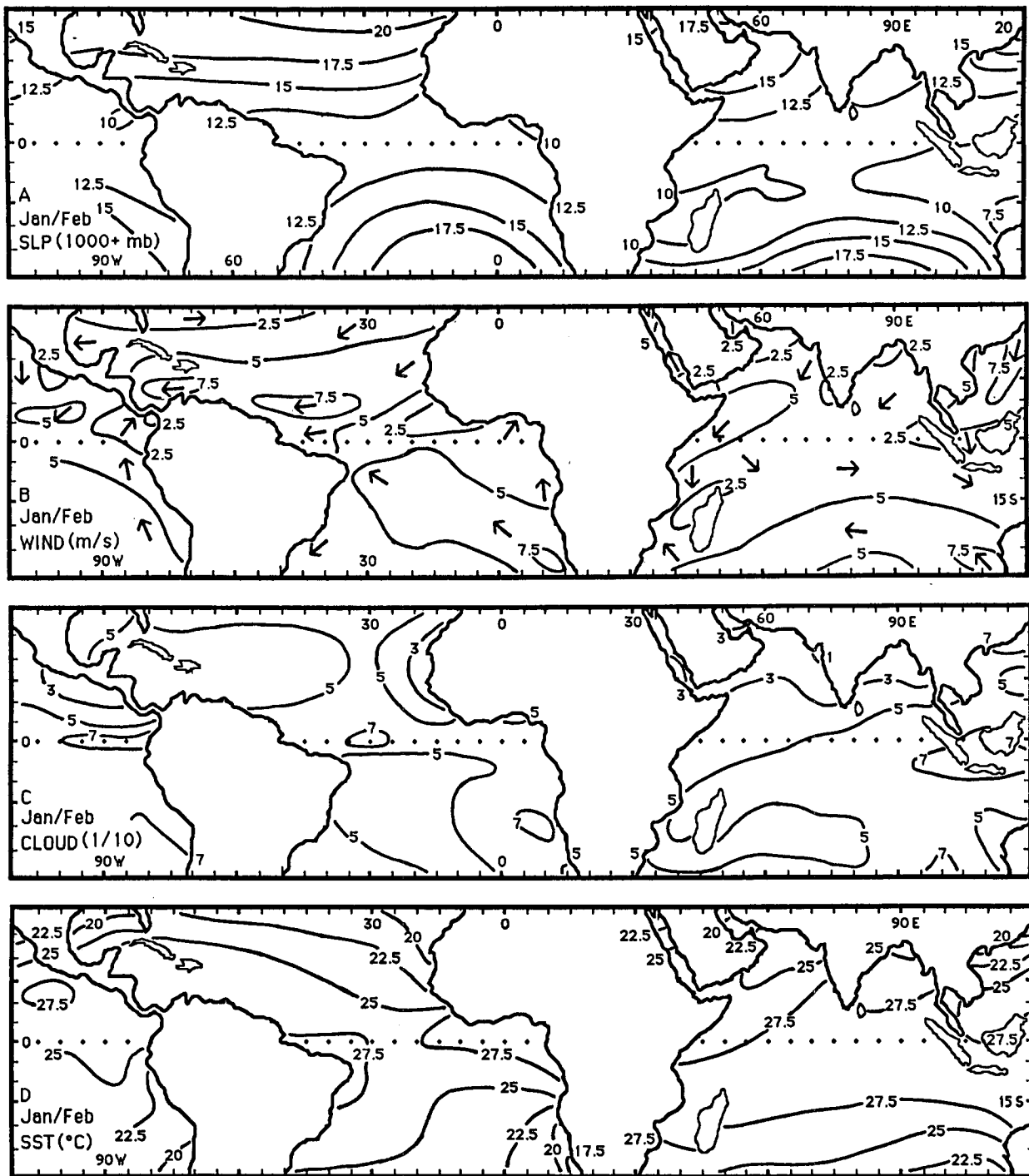
FIG. 2. January/February mean fields (1948-83) of a) sea-level pressure, in (1000+)mb, b) wind speed, in \text{m s}^{-1} , and selected directional wind arrows, c) total cloudiness, in tenths, and d) sea surface temperature, in ^{\circ}\text{C} .
