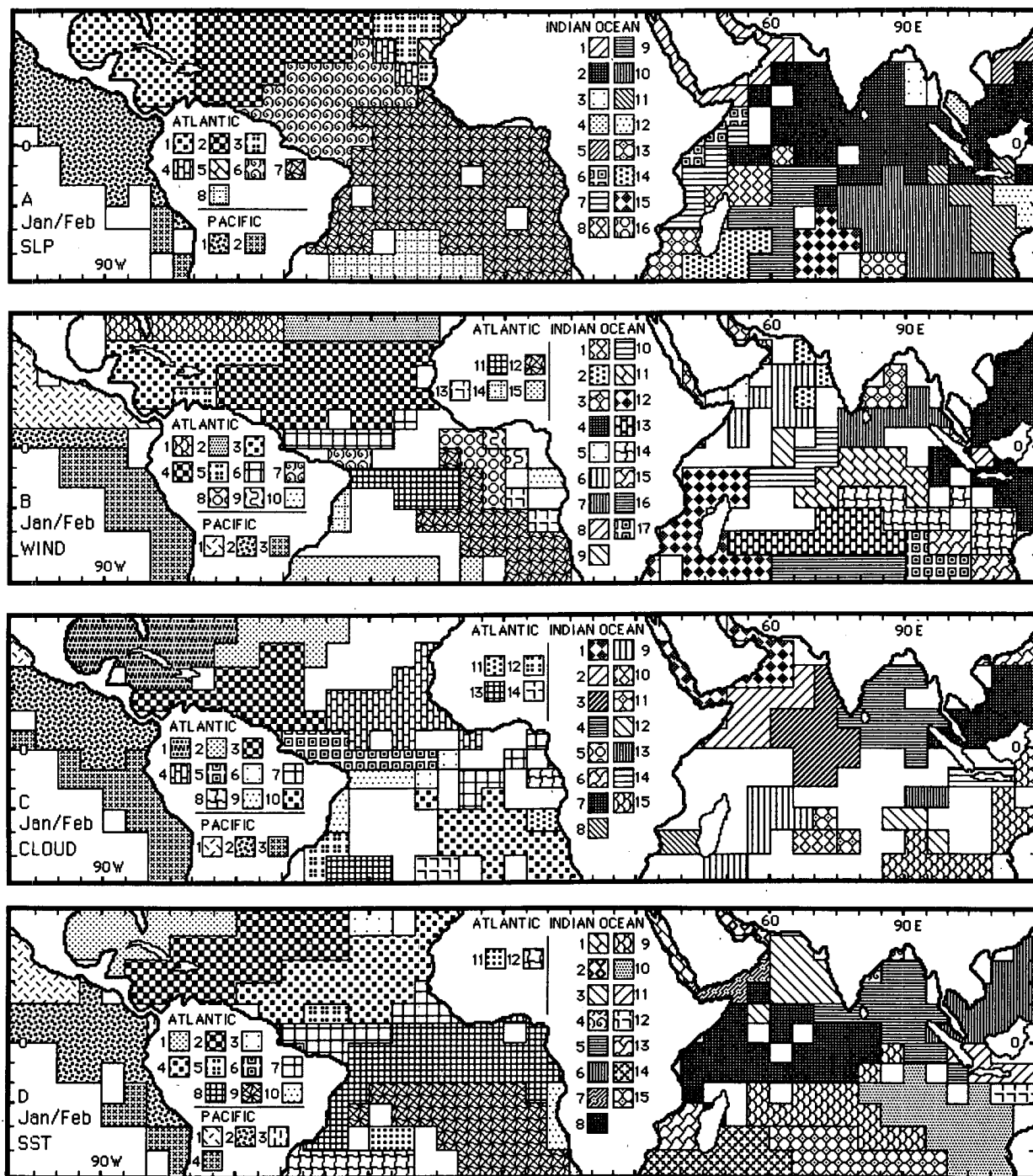
FIG. 6. January/February \beta -cluster distribution maps (1948–83) of a) sea-level pressure, b) wind speed, c) total cloudiness, and d) sea surface temperature. In each map legend, all patterns are listed with their ocean domain (P Pacific, A Atlantic, and I Indian Ocean) and code number. Similar patterns depict related clusters within each map (i.e., members of the same \alpha - or \beta -cluster); enhanced patterns represent strong clusters.
