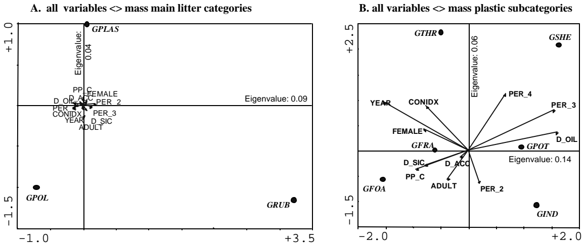
Figure 5. Examples of biplots resulting from CANOCO analyses, in this case showing relationships between mass of litter in Fulmar stomachs (dependent variables, circles with italics text) and potentially relevant independent variables (arrows, normal text). Axes are significant but have very low Eigenvalues (shown along inner axes). See methods for acronyms used. Examples of interpretation: in B. the long arrow for the variate year in the opposite direction of the position of mass of industrial plastics ( GIND ) suggests a negative relation between increasing years and industrial plastics; the short arrow for factor plumage colour suggests relatively weak differences between coloured birds ( PP_C ) and white birds in the centerpoint of the graph: the arrow direction towards mass of foamed plastics ( GFOA ) could suggest a weak positive relationship between arctic origin and foamed plastic.
