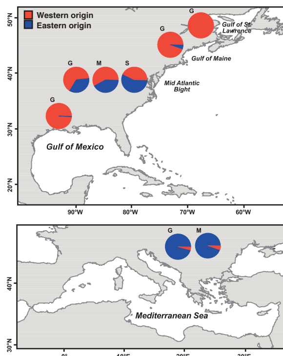
Fig. 3. Estimates of natal origin for school (S), medium (M), and giant (G) category Atlantic bluefin tuna from spawning areas (Mediterranean Sea, Gulf of Mexico) and foraging areas (Gulf of St. Lawrence, Gulf of Maine, Mid Atlantic Bight). Contribution rates (percentages) were determined by comparing milled otolith cores (corresponds to yearling period) to a baseline sample from eastern and western nurseries (east + west = 100%). Assignment to either eastern or western nursery was based on maximum likelihood estimations. Standard deviations (SD) were expressed as percentages of estimated proportions. Size classes were approximated based on weight or age (actual or derived from length): giant (>140 kg, \geq age 10 years), medium (60 to 140 kg, age 5 to 9 years), and school (<60 kg, < age 5 years) category bluefin tuna. Percentage contribution of "western population" and standard deviation (SD) around estimated proportion per region and size category: Gulf of Mexico [giant: 99.3% (SD 1.7%), n = 42 ]; Mediterranean Sea [giant: 4.2% (SD 3.1%), n = 94 ; medium: 4.2% (SD 4.4%), n = 38 ]; Gulf of St. Lawrence [giant: 100% (SD 0.0%), n = 38 ]; Gulf of Maine [giant: 94.8% (SD 5.3%), n = 72 ]; Mid Atlantic Bight [giant: 64.9% (SD 21.9%), n = 12 ; medium: 55.7% (SD 10.4%), n = 56 ; school: 42.6% (7.2%), n = 86 ].
