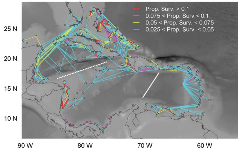
Fig. 4. Connectivity network for reef fish populations in the wider Caribbean plotted for various levels of larval exchange (proportion surviving) between each reef site (or node N_i , where center location is represented by a small gray circle; note that there is no directionality represented in the exchange). Two major meridional biogeographic breaks are identified: one in the eastern Caribbean Sea (white line) and the other one at the northern edge of the Nicaraguan Rise (dotted white line), which separate the eastern and western Caribbean. Two enclaves stand out: the Bahamas Bank, including the Turks and Caicos Islands, and the Nicaraguan Archipelago, which are both strongly intraconnected. The Panama-Colombian Gyre subregion is also largely isolated from the rest of the Caribbean, with little connection between Panama and Colombia. Note that connections at levels below 0.05% (proportion surviving) are not likely contributing appreciably to ecological connectivity but are shown here because they may become important when accumulated from different sources at one particular location.
